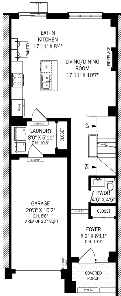
MAIN FLOOR - 687 SQUARE FEET
